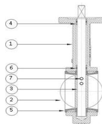
Fig. 1 — Component identification, numbered per table.
