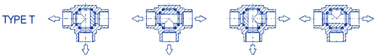
Type T ball — four handle positions and the resulting flow paths.
