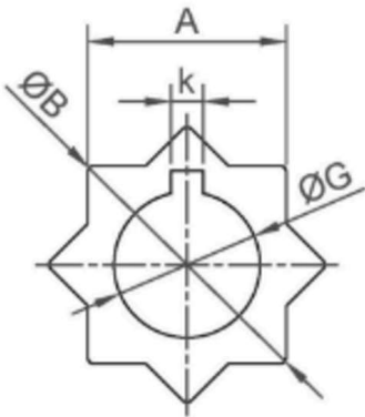
A across flats, ØB over star points, ØG bore and k key way width.
